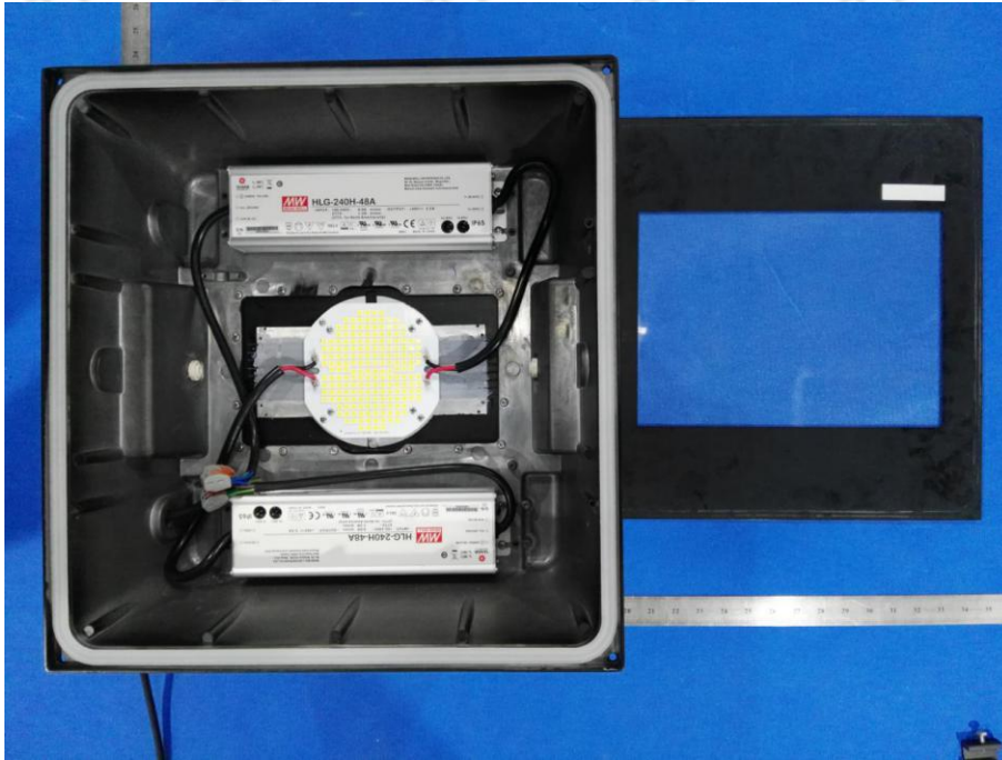
Fig.5 – Inner view
