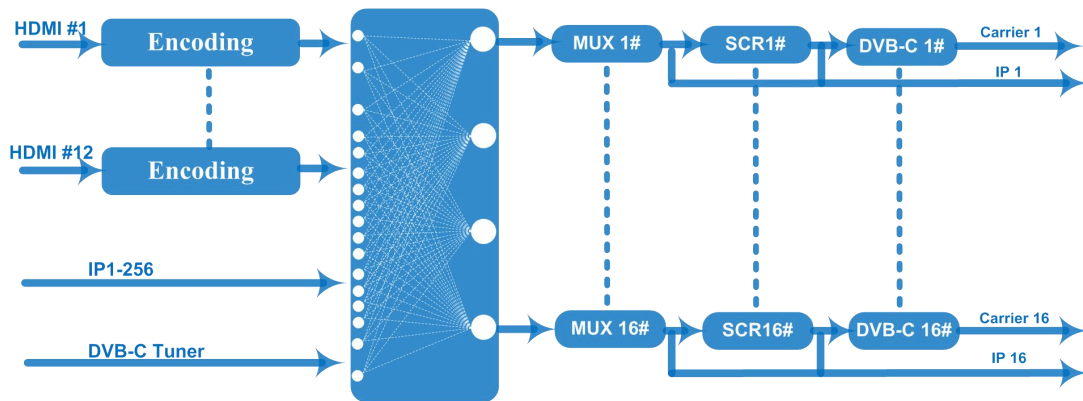
DVB-C Principle Chart
