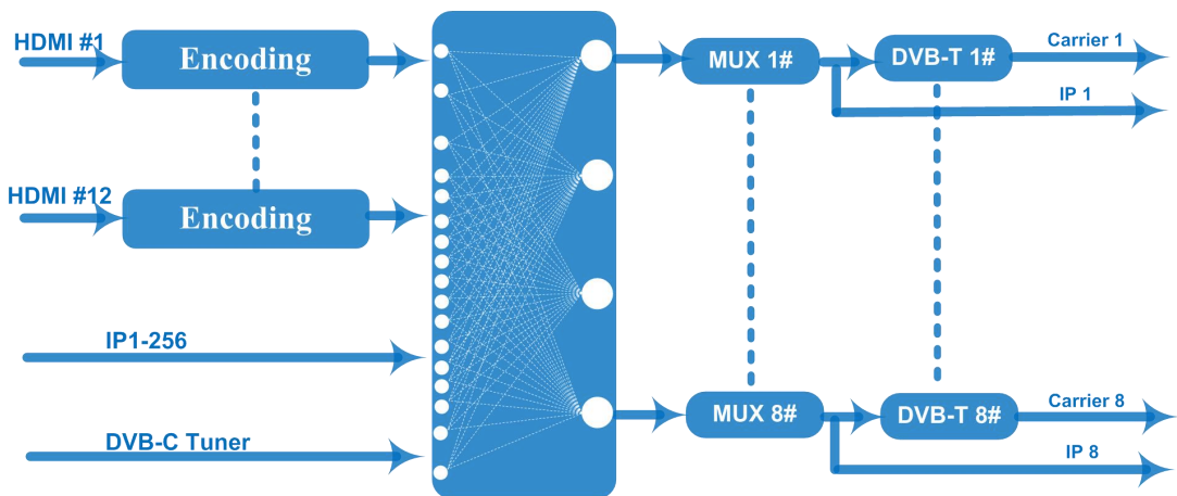
DVB-T Principle Chart
