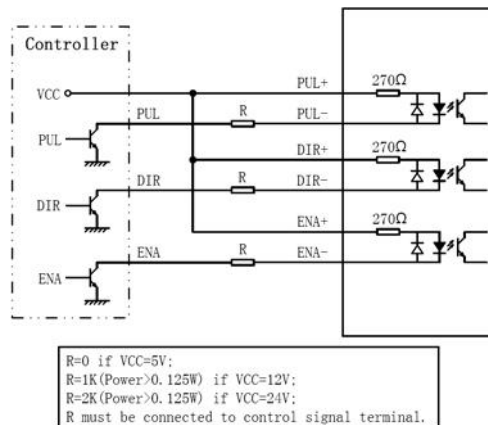
Figure 3: Connections to open-collector signal (common-anode)
