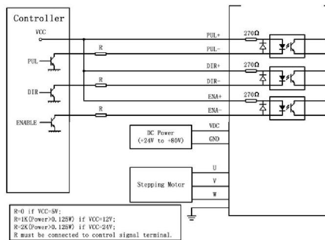
Figure 6: Typical connection
