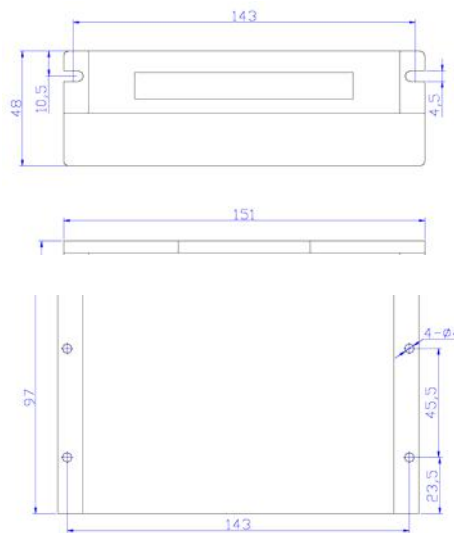
Figure 1: Mechanical Specifications
